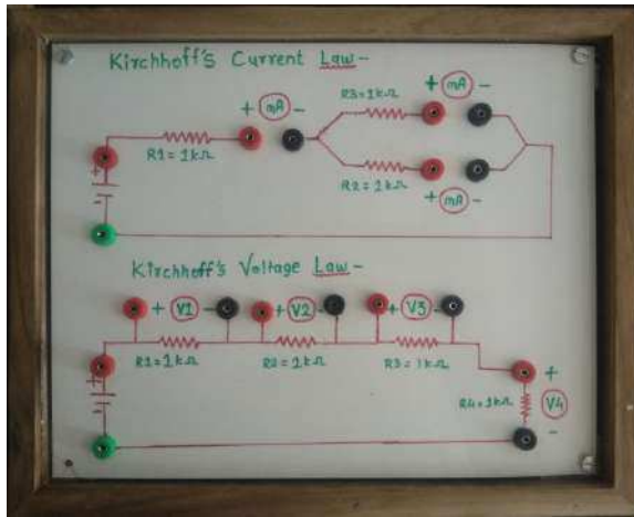
Picture 2. KVL-KCL kit
